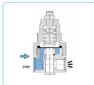
with diaphragm
