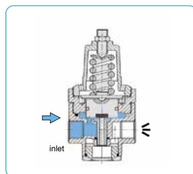
with piston
