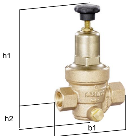
DN 15 - DN 32
