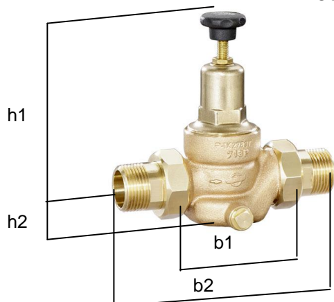
DN 15 - DN 32
