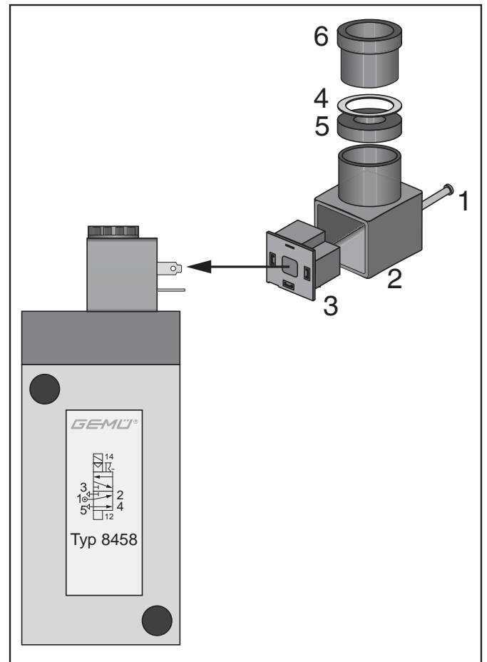
Electrical connection
